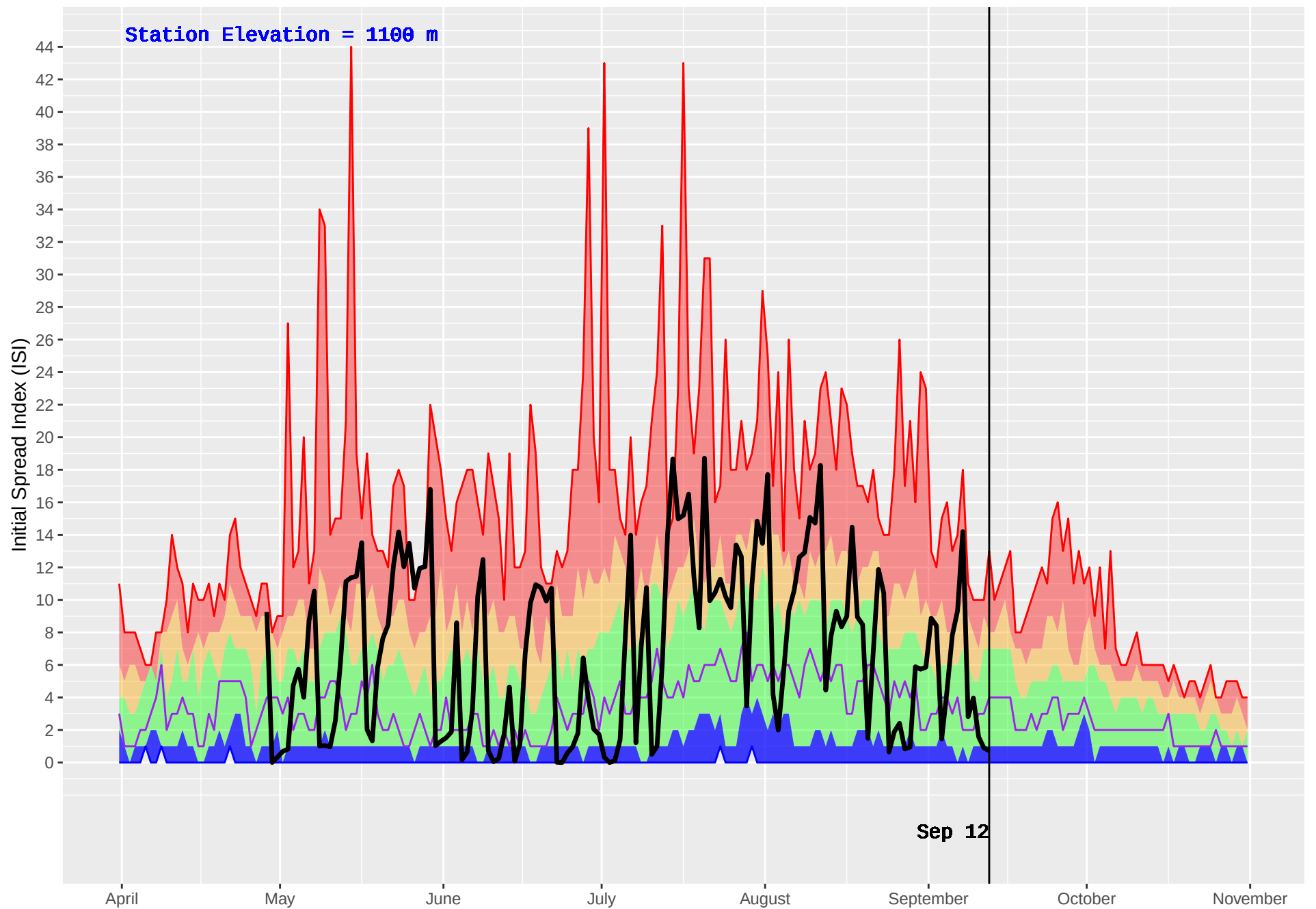
PALLISER (411) : Historical (1973–2016) and Current (2018) Daily Initial Spread Index (ISI)
