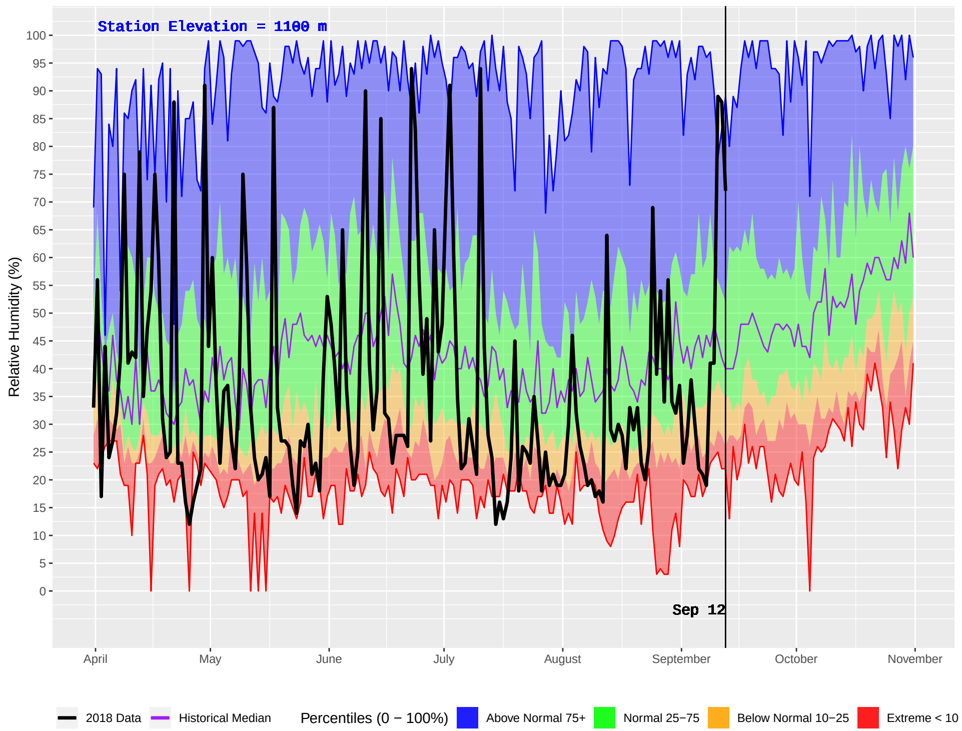
PALLISER (411) : Historical (1973–2016) and Current (2018) Daily Relative Humidity
