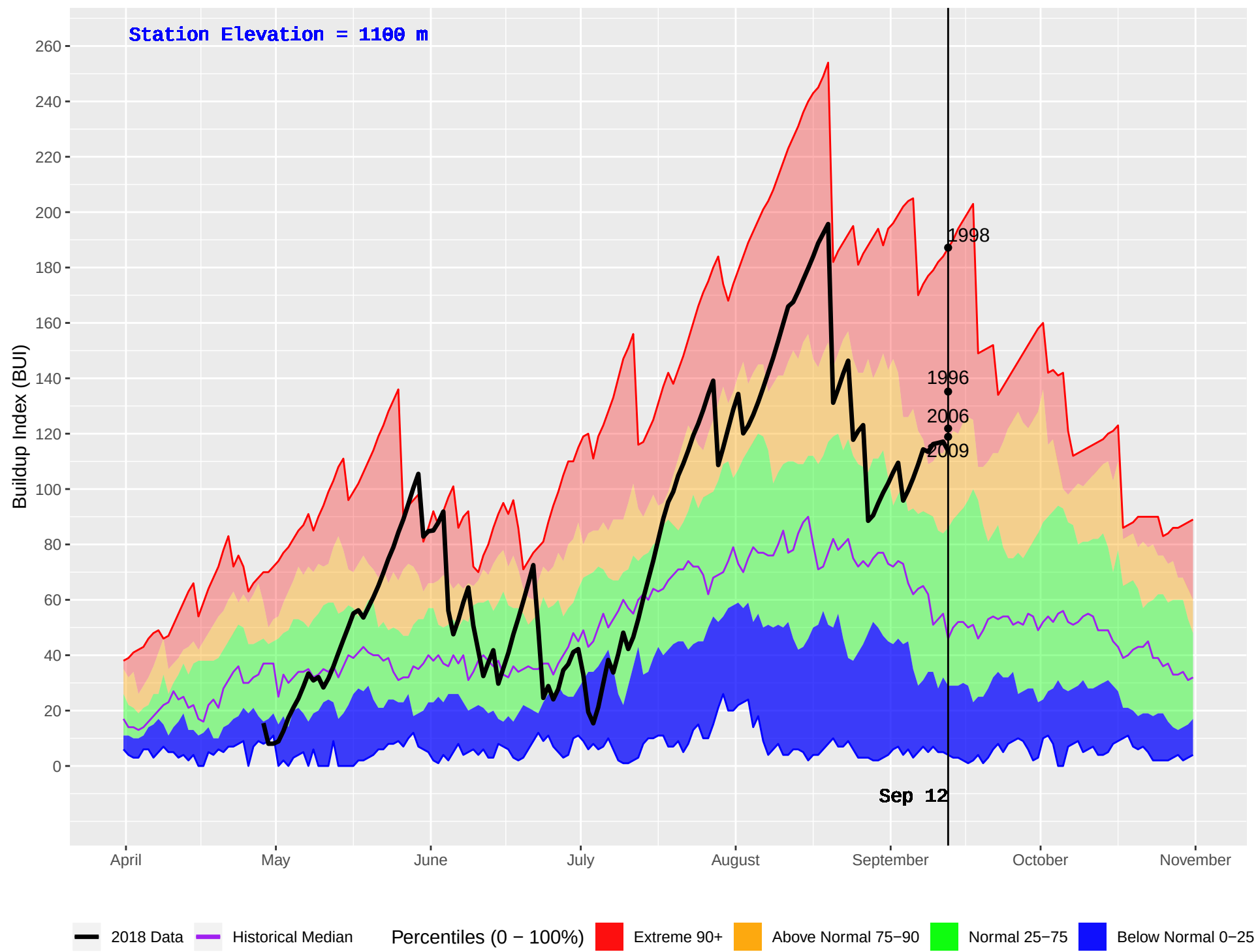
PALLISER (411) : Historical (1973–2016) and Current (2018) Daily Buildup Index (BUI)
