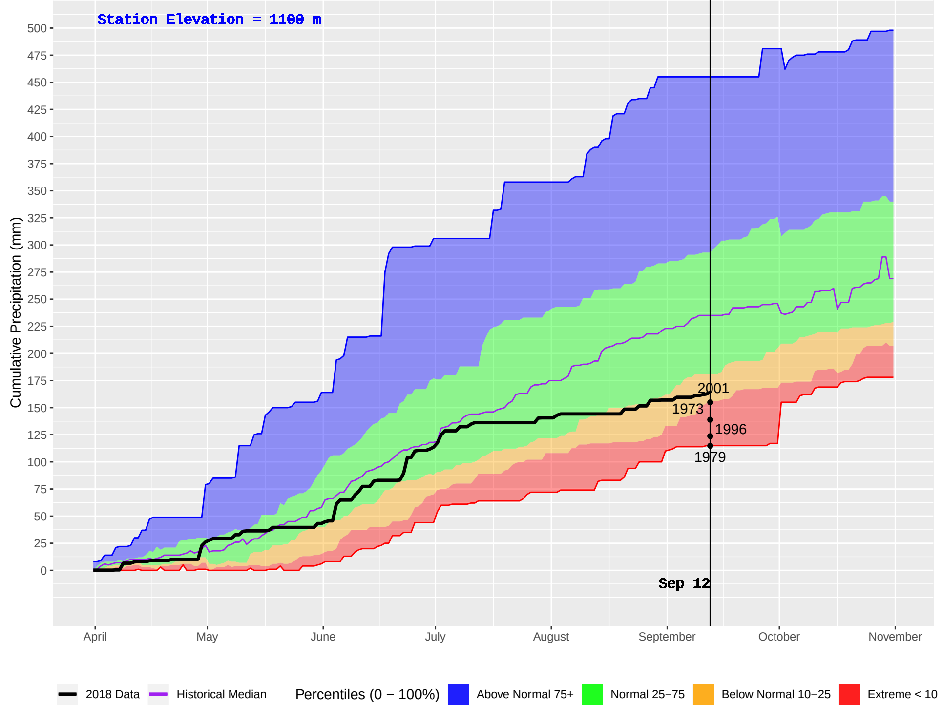
PALLISER (411) : Historical (1973–2016) and Current (2018) Daily Cumulative Precipitation
