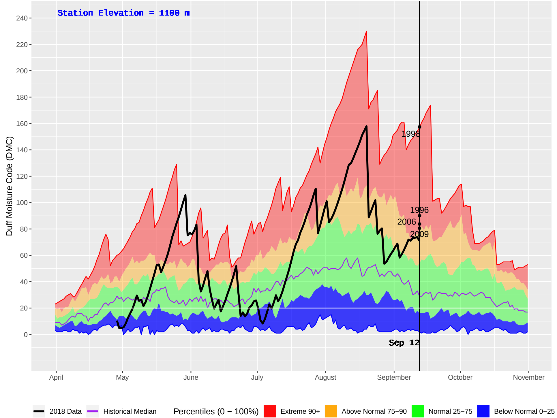
PALLISER (411) : Historical (1973–2016) and Current (2018) Daily Duff Moisture Code (DMC)
