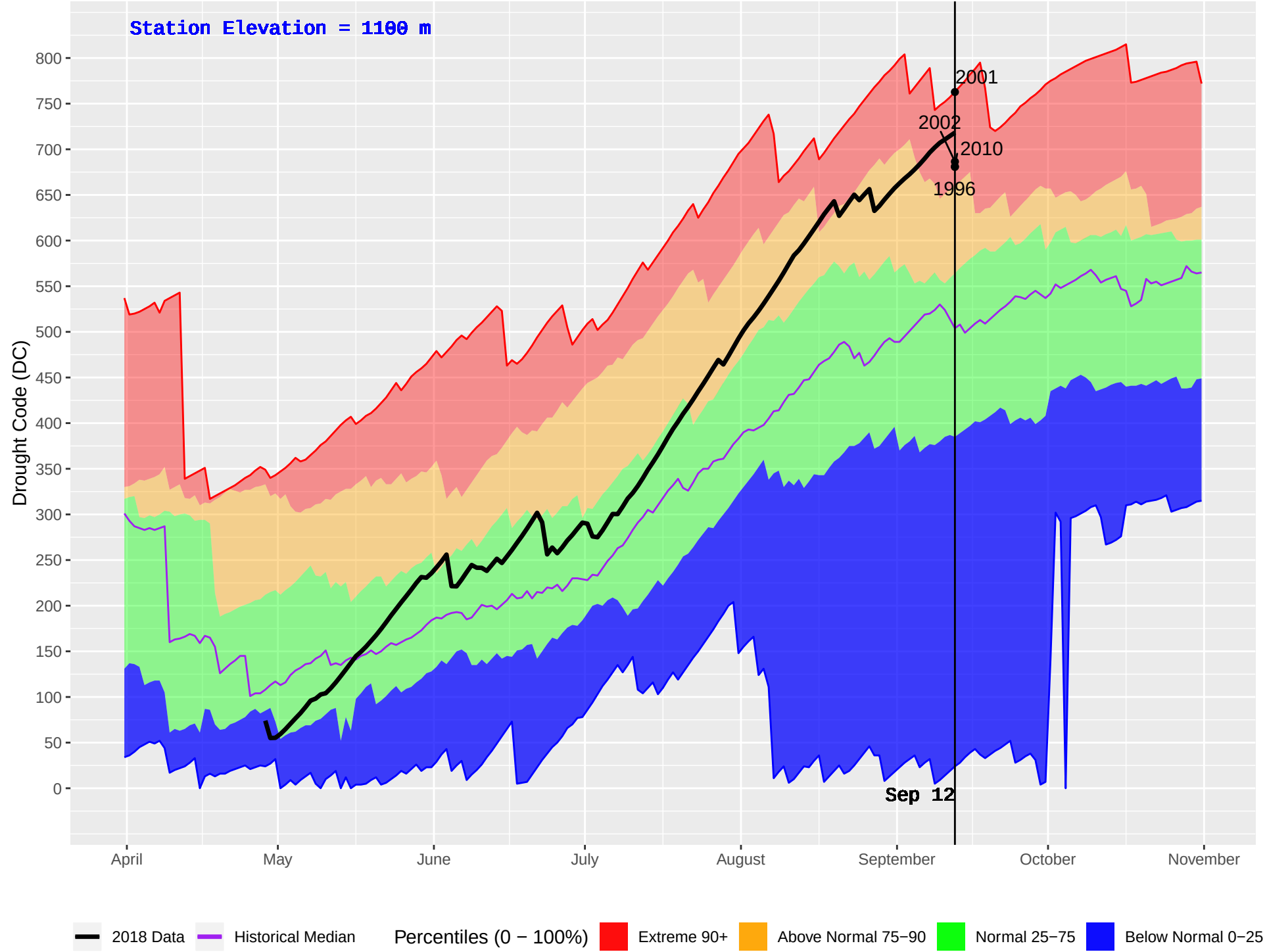
PALLISER (411) : Historical (1973–2016) and Current (2018) Daily Drought Code (DC)
