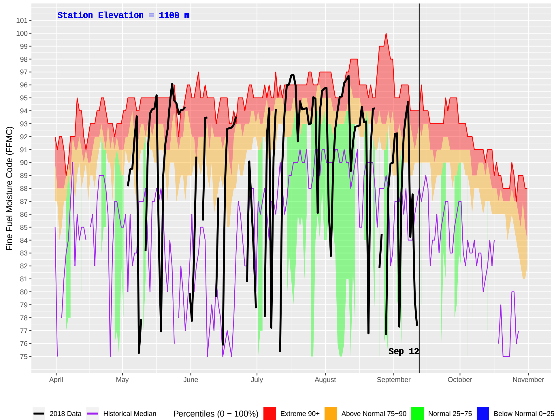
PALLISER (411) : Historical (1973–2016) and Current (2018) Daily Fine Fuel Moisture Code (FFMC)
