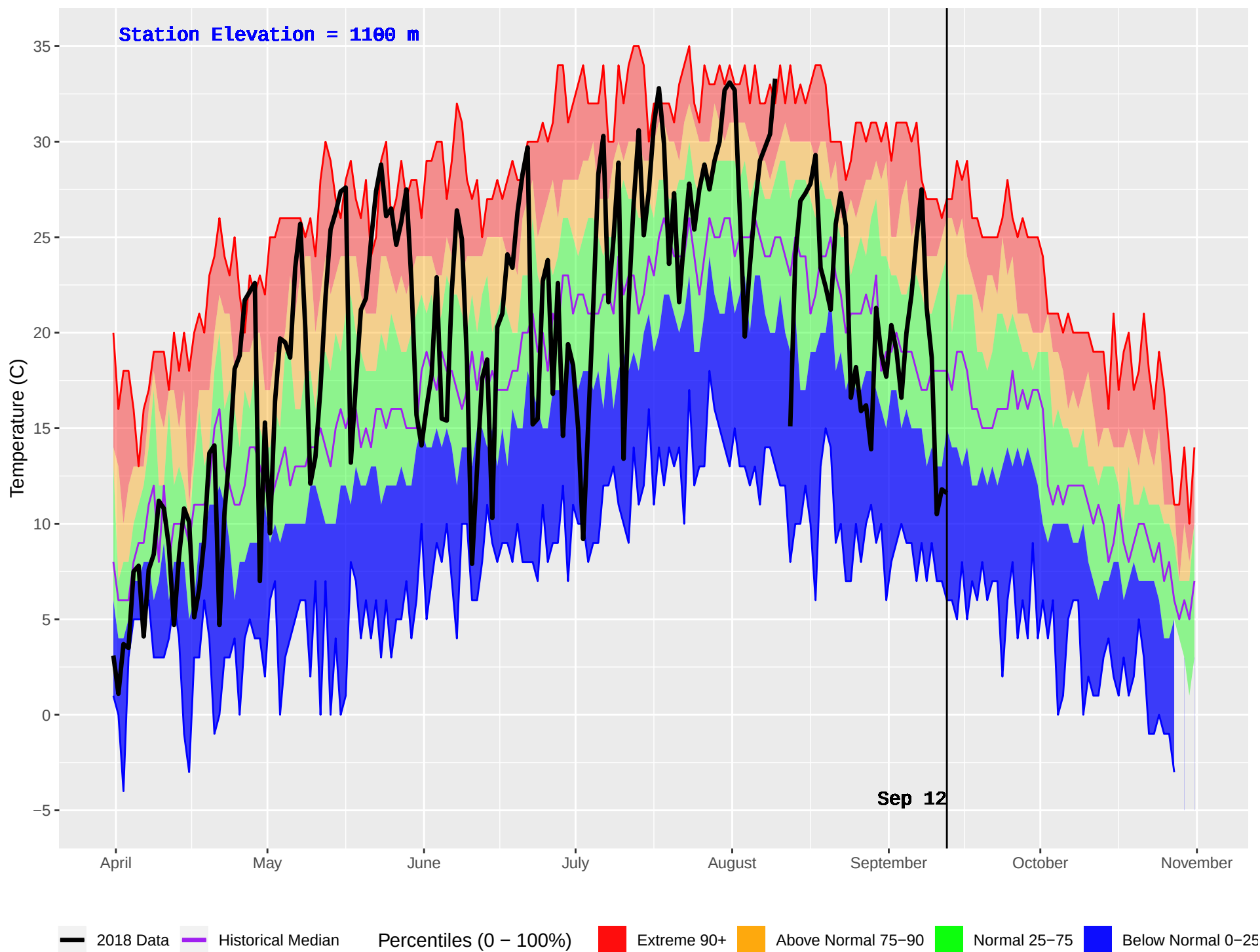
PALLISER (411) : Historical (1973–2016) and Current (2018) Daily Temperature
